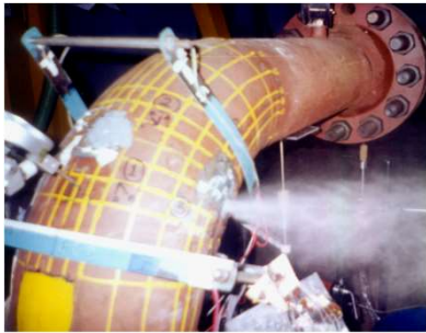
Failed elbow due to Ratcheting-Fatigue
