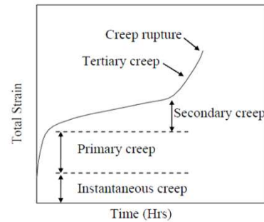
Creep deformation process
