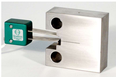
Assessment & Testing for Fracture and Fatigue Crack Growth
